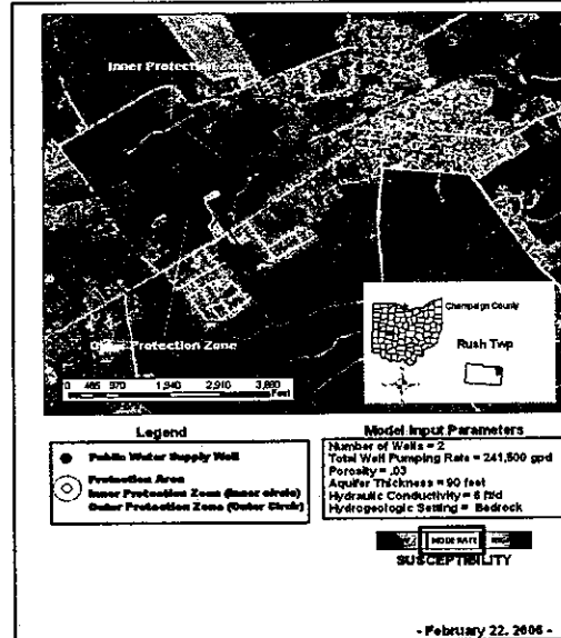
Figure 1. Drinking Water Source Protection Area Village of North Lewisburg Public Water System Identification Number 1109012
